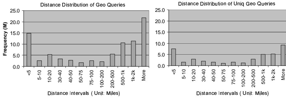
Figure 2: Distributions of the distance L between the city Q_c in the query and the issuer's IP location. X axis denotes the distance intervals used (less than 5 miles, 5-10 miles, etc), Y axis denotes the number of geo queries (unit: million) in each interval. Left/Right graph shows L 's distribution in the geo sub training set before/after we remove the duplicates respectively.
