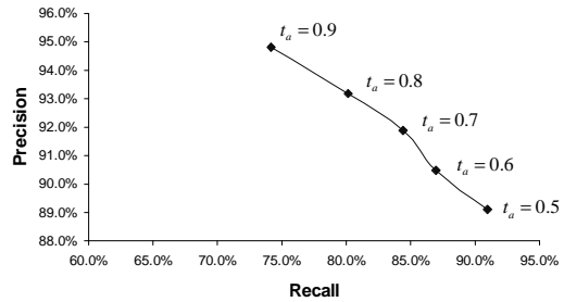
Figure 3: Precision/Recall curve on training subset III for location-specific query discovery.
